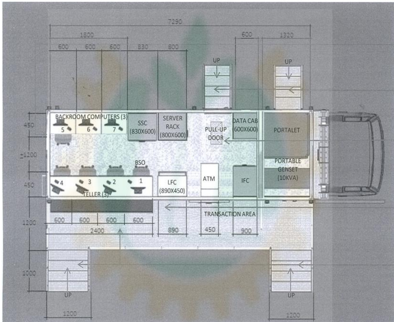
INSIDE VIEW
