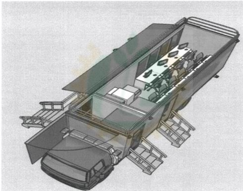
ISOMETRIC VIEW
