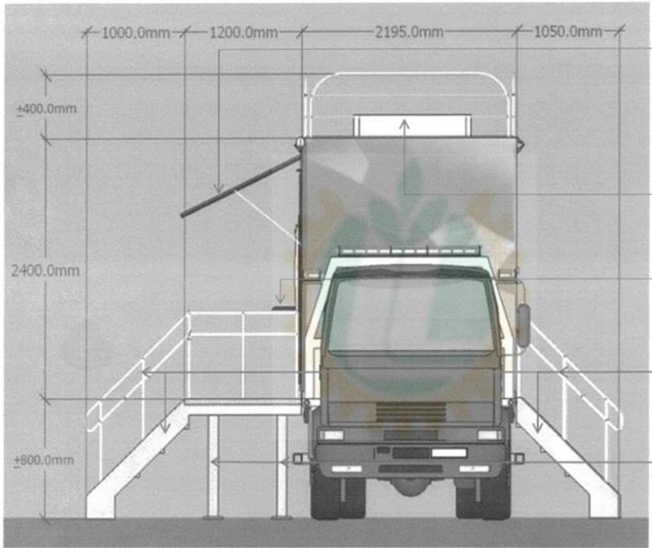
FRONT VIEW
